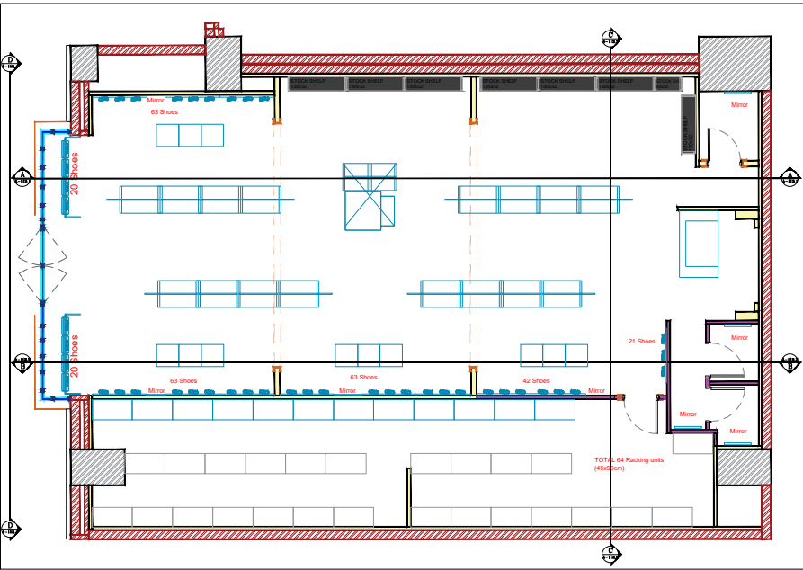
A 113.1 Elevation A-A Key plan
