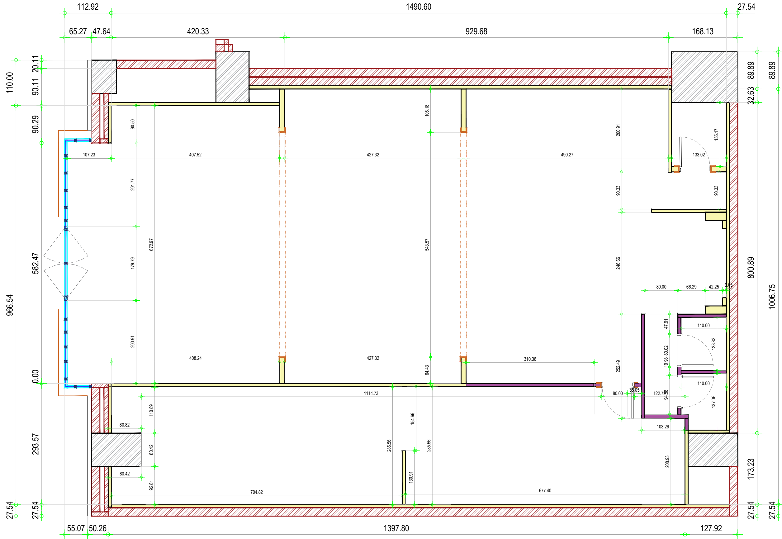
A 106 Construction plan
